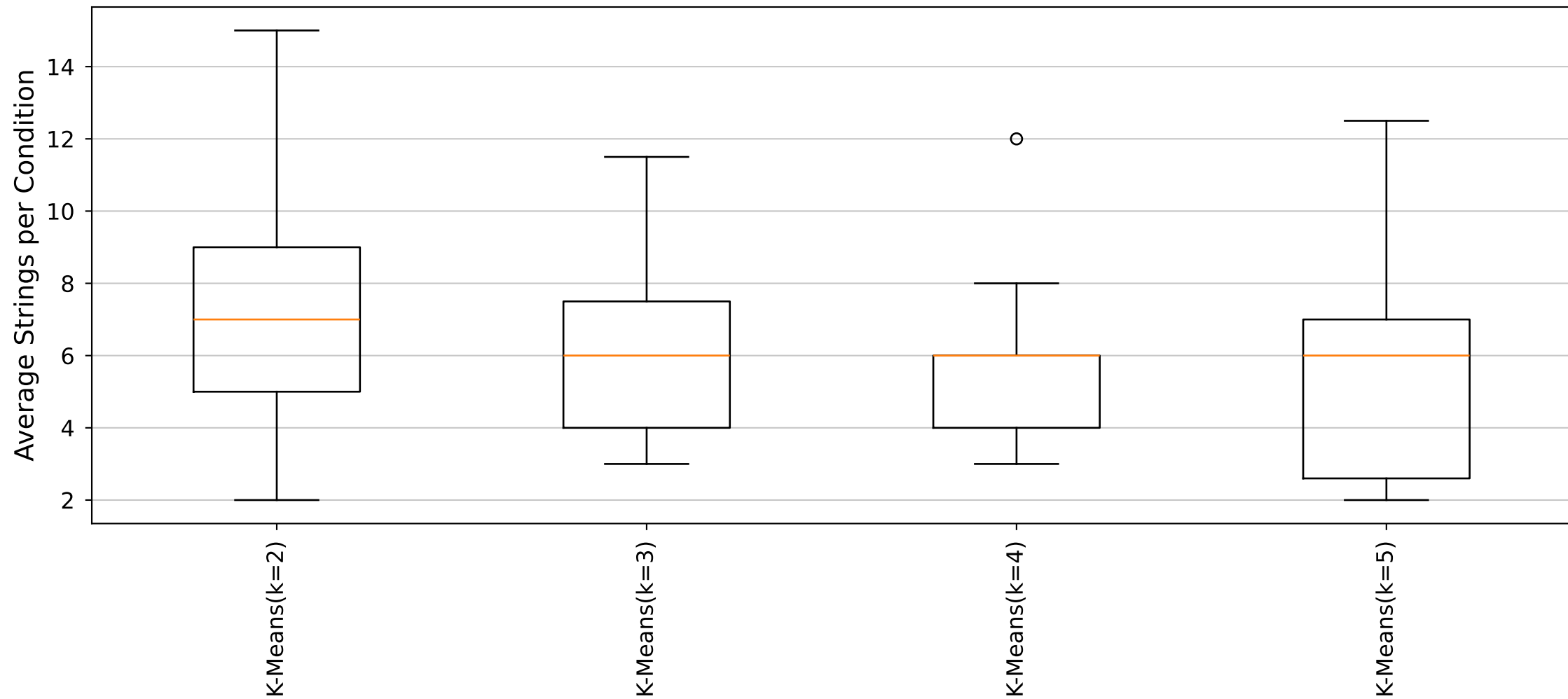
YARA Rules Average Strings per Condition Distribution (Cluster45_Size5 dataset)
